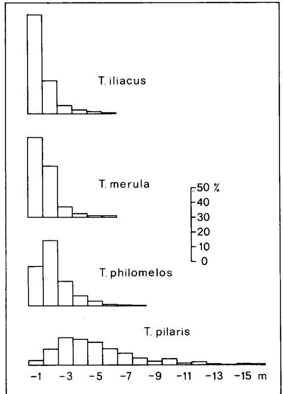
FIG. 2. Height above the ground of the nests of four thrush species, according to data in v. HAARTMAN (1969).
