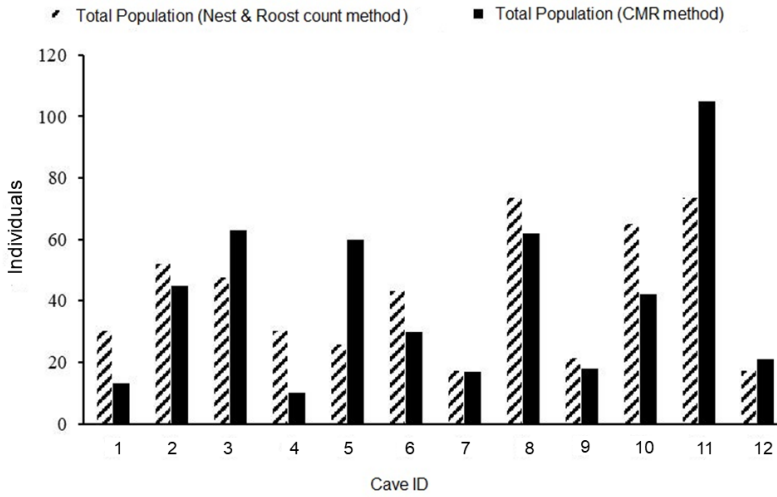
Fig. 3. Population estimation using total population (Nest & Roost Count Method) and Total population (CMR method) in the study caves.
