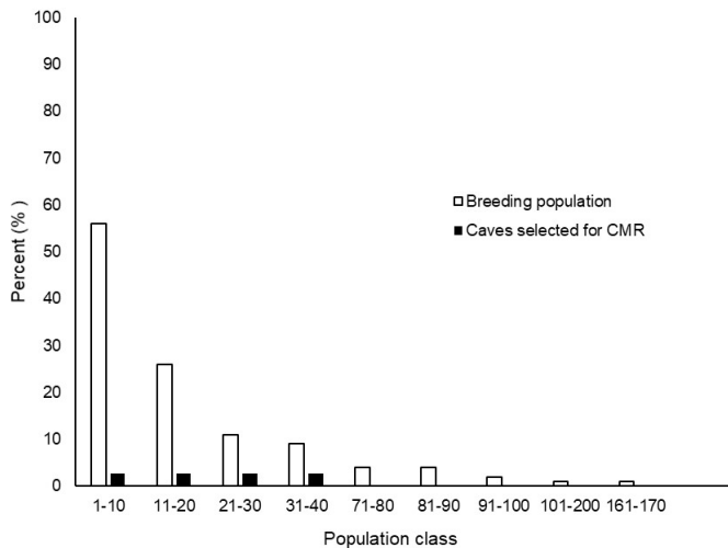
Fig. 2. Caves in Baratang classified based on breeding population, with three caves from each class (0–10, 11–20, 21–30, and 31–40 pairs) selected for Capture-Mark-Recapture.
