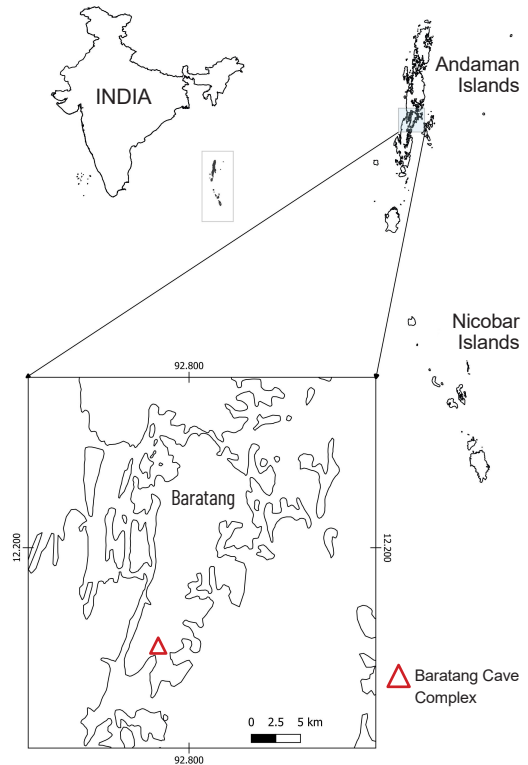
Fig. 1. The geographic location of the study area (Baratang Cave Complex) in the Andaman Islands.
